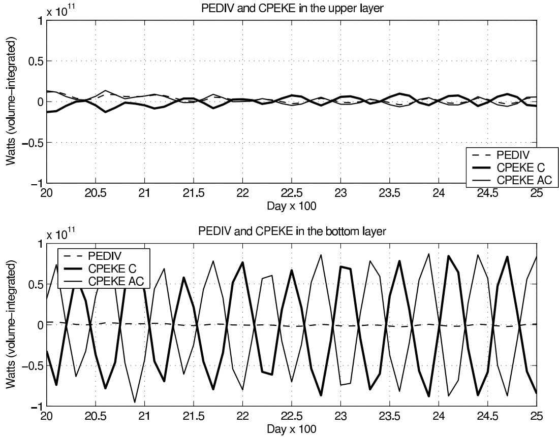
Figure 2.11: PEDIV (dashed line) and (CPEKE) during the equilibrium in the upper layer (upper panel) and the bottom layer (bottom panel). Thicker(thinner) line is CPEKE in the cyclonic(anticyclonic) gyre.
