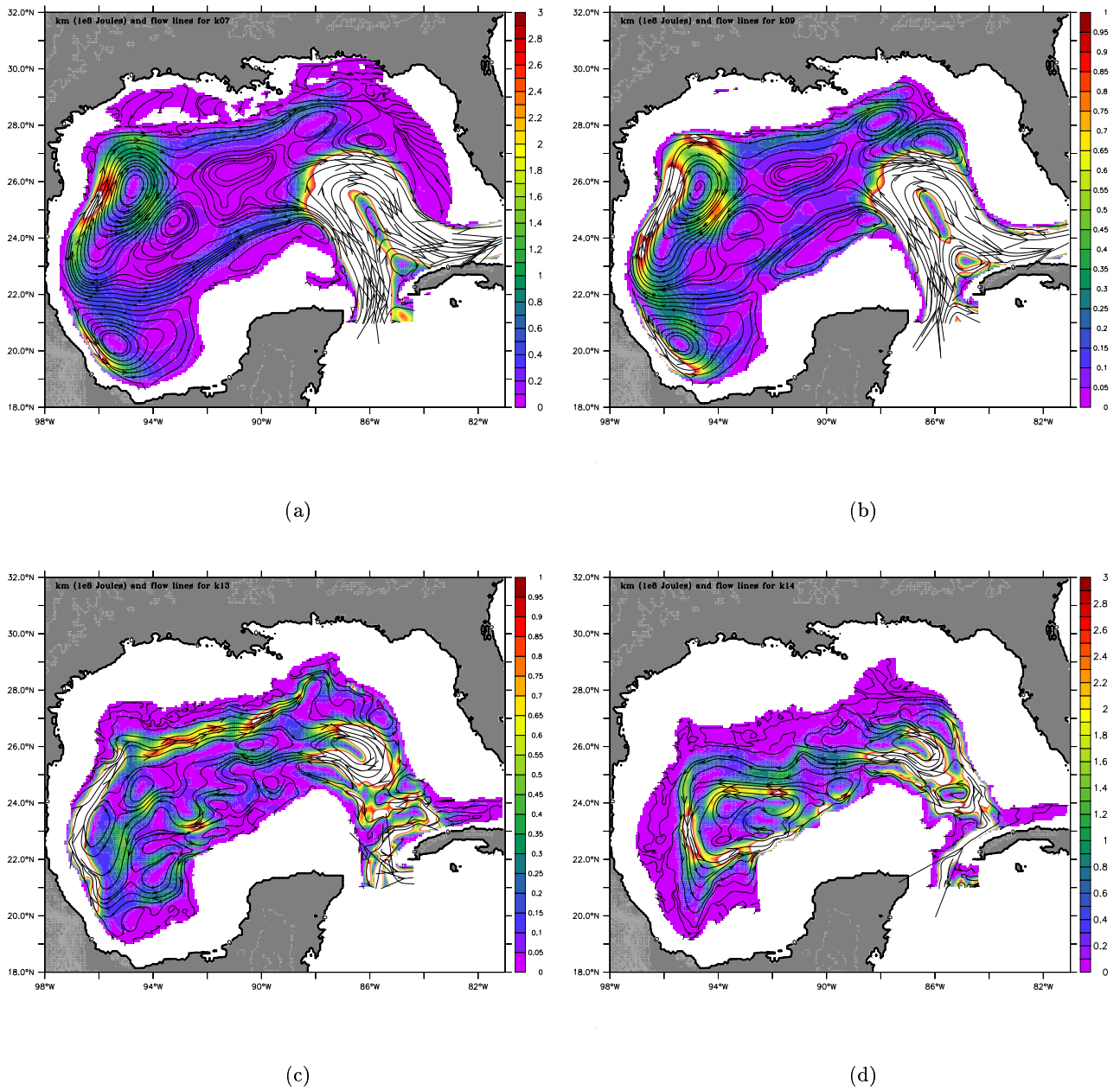
Figure 5.3: 7years-averaged, volume-integrated kinetic energy of the mean flow, KM , at four model layers ( 10^8 Joules). (a) Layer 7 ( \sim 300 m depth), (b) layer 9 ( \sim 700 m depth), (c) layer 13 ( \sim 1700 m depth), and (d) layer 14 (below 2000m in average).
