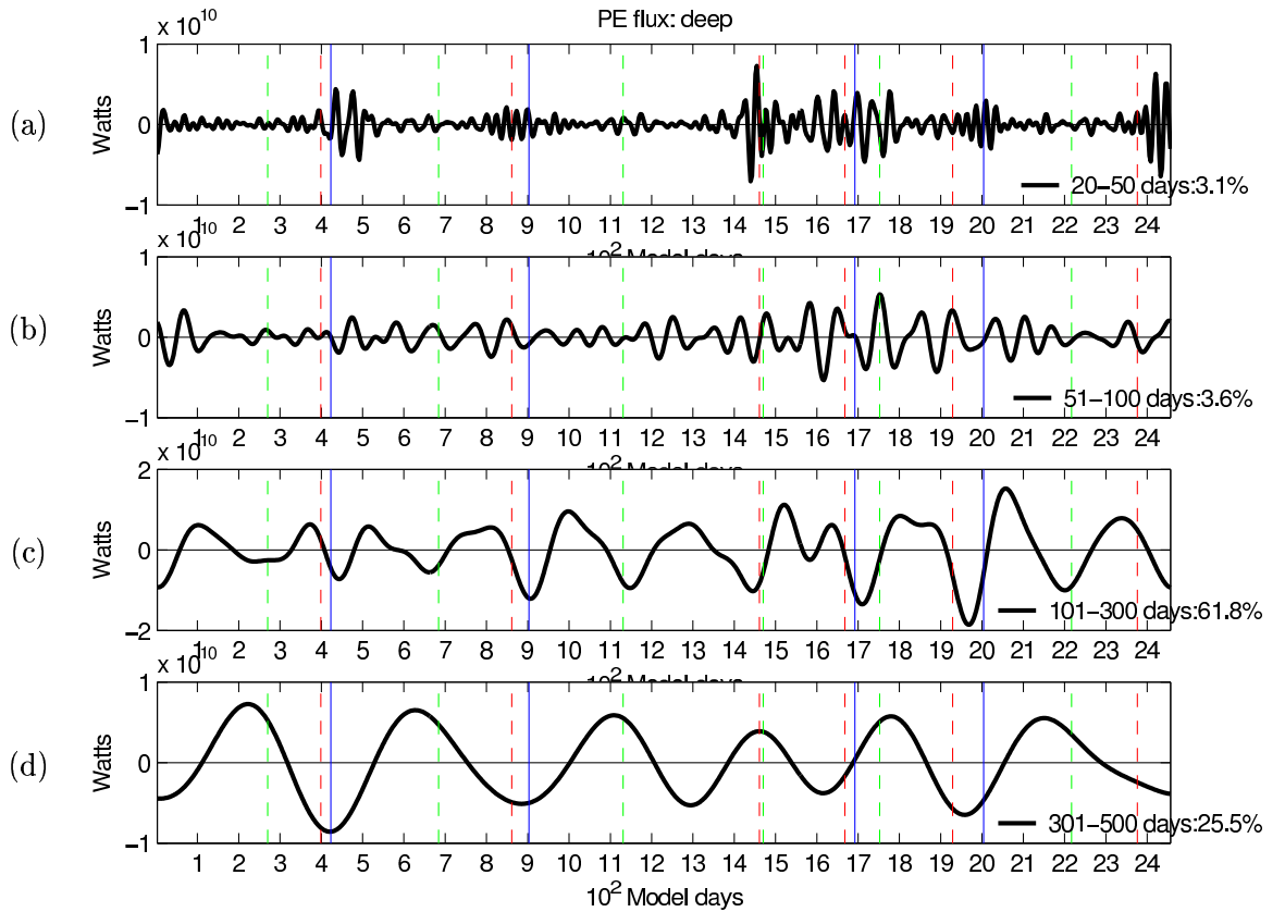
Figure 4.4: Variability of the potential energy flux ( PE_{flux} ) across 89W in deep waters ( >2000\text{m} in average). Blue solid vertical lines represent a LC port-to-port position; green dashed vertical lines represent LC intrusions beyond 25N; red dashed vertical lines represent ring shedding events. (a) band 20-50 days: 3.1%; (b) band 51-100 days: 3.6%; (c) band 101-300 days: 61.8%; (d) band 301-500 days: 25.5%.
