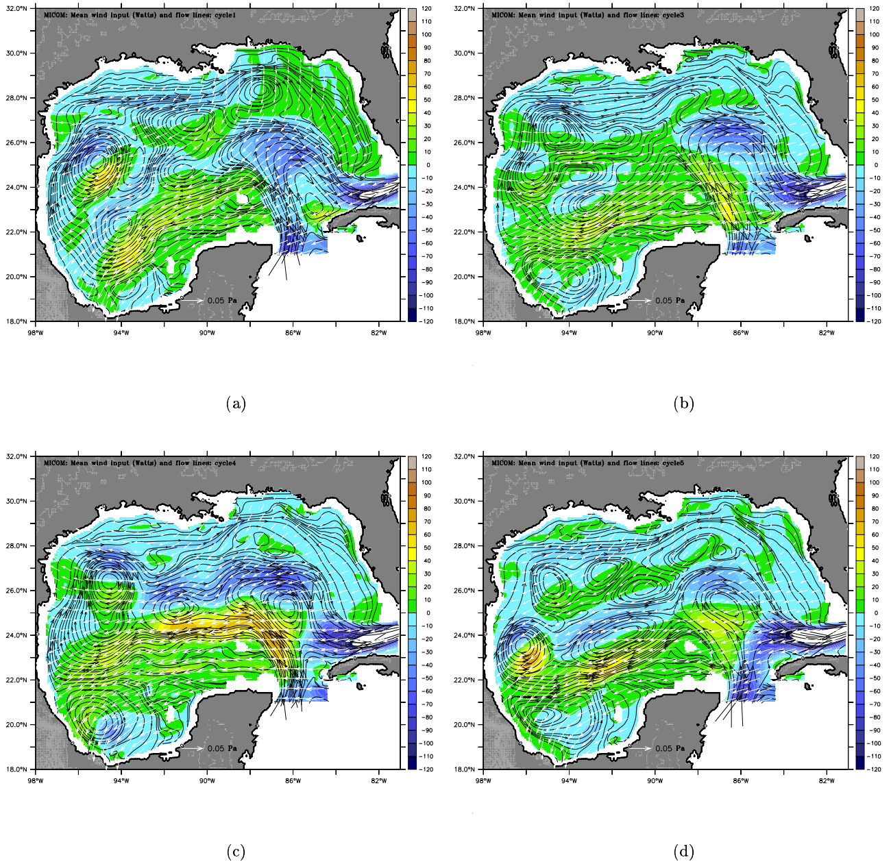
Figure 4.10: Time-averaged wind input into the Gulf of Mexico during four Loop Current cycles (Watts). Vectors are mean wind stress (Pa) computed from the ECMWF dataset (1980-1986); the color scale (Watts) is time-averaged work done by the wind on surface currents [ MWIND , equation (15)]. Green-yellow-red colors are positive work, and represent regions where the mean surface flow is locally wind-intensified. Blue tones stand for areas where the mean surface currents do work against the wind stress. Flow lines are surface currents within the mixing layer. (a) cycle 1, (b) cycle 3, (c) cycle 4, (d) cycle 5.
