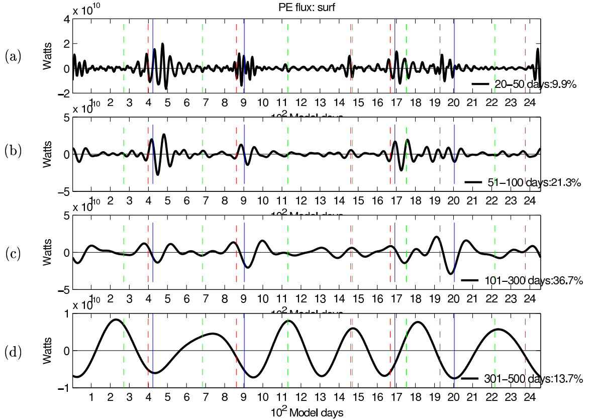
Figure 4.3: Variability of the potential energy flux ( PE_{flux} ) across 89W in surface waters (upper 500m in average). Blue solid vertical lines represent a LC port-to-port position; green dashed vertical lines represent LC intrusions beyond 25N; red dashed vertical lines represent ring shedding events. (a) band 20-50 days: 9.9%; (b) band 51-100 days: 21.3%; (c) band 101-300 days: 36.7%; (d) band 301-500 days: 13.7%. About 20% of the variability occurs at periods larger than 500 days (not shown).
