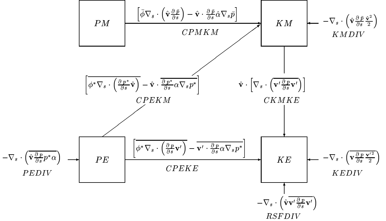
Figure 2.2: Energy diagram in isopycnic open systems [adapted from Bleck, 1985 ]. The direction of the arrows is controlled by the sign of the energy terms. Terms beginning with C stand for energy transfers, while terms ending in DIV represent energy boundary fluxes. For simplicity, energy inputs and energy dissipation in each box are omitted.
