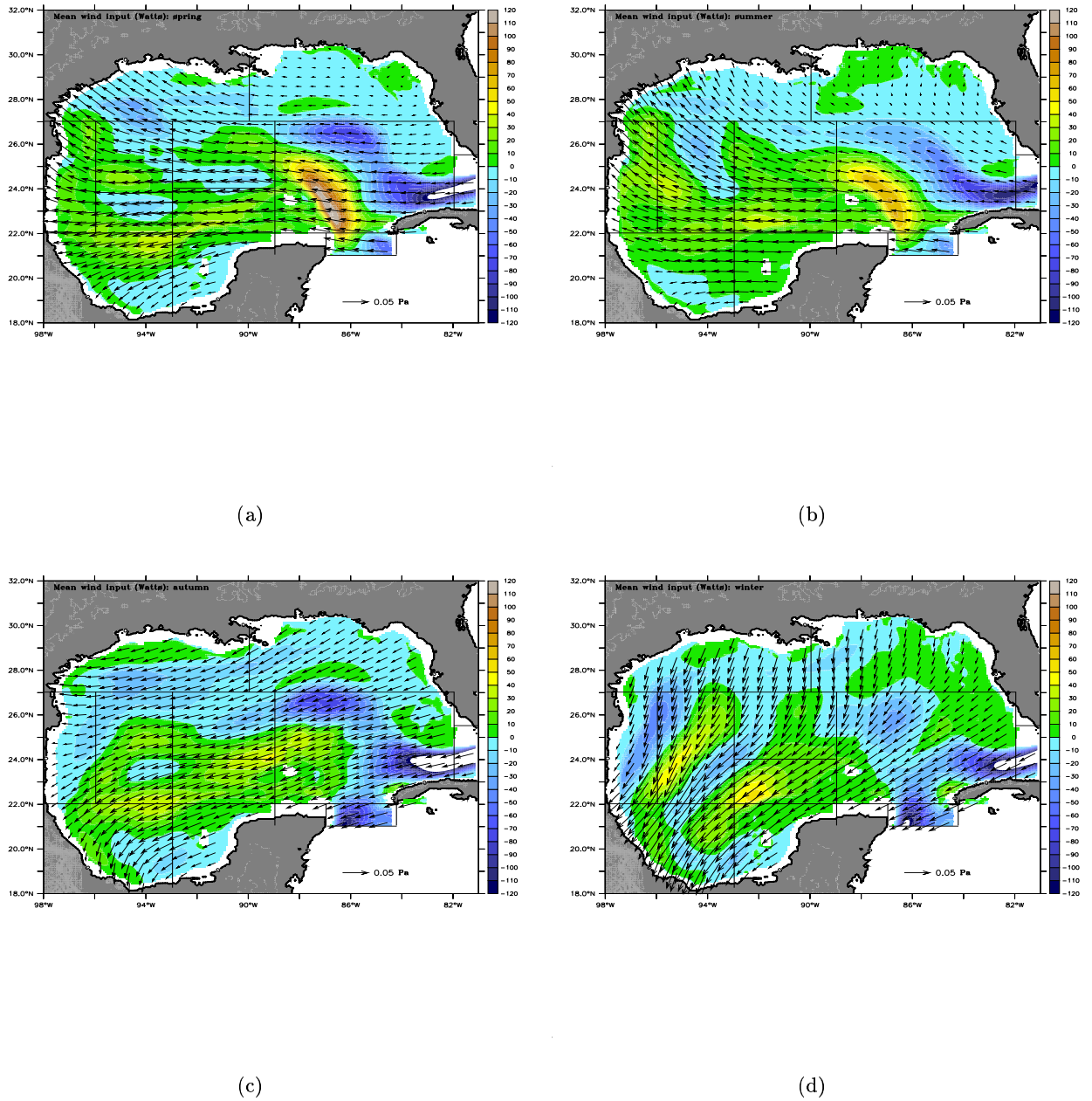
Figure 4.1: Seasonal wind input into the Gulf of Mexico for the 7-years of the experiment. Vectors are mean wind stress (Pa) computed from the ECMWF dataset (1980-1986); the color scale (Watts) is time-averaged work done by the wind on surface currents [ MWIND , equation (15)]. Green-yellow-red colors are positive work, and represent regions where the mean surface flow is locally wind-intensified. Blue tones stand for areas where the mean surface currents do work against the wind stress. (a) Spring, (b) summer, (c) autumn, (d) winter.
