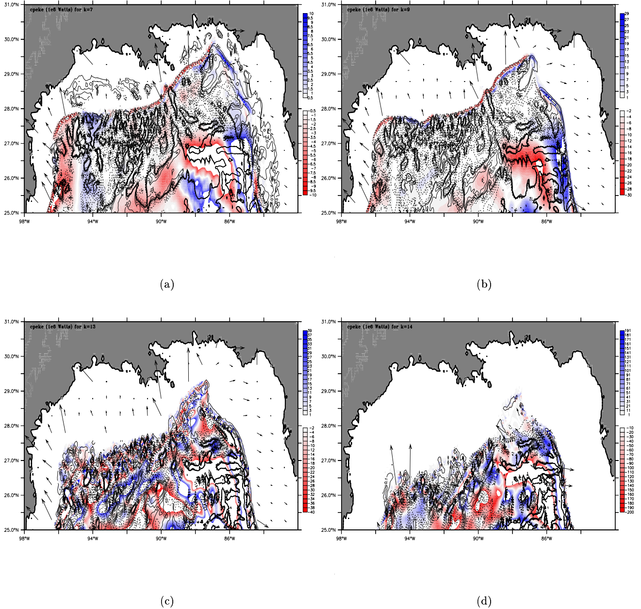
Figure 5.7: 7years-averaged CPEKE (color scale in 10^6 Watts) and Reynolds stress (contours) at the Northern Gulf of Mexico. The arrows indicate the orientation of the local \beta -north. (a) Layer 7 (~300m depth), (b) layer 9 (~700m depth), (c) layer 13 (~1700m depth), and (d) layer 14 (below 2000m in average).
