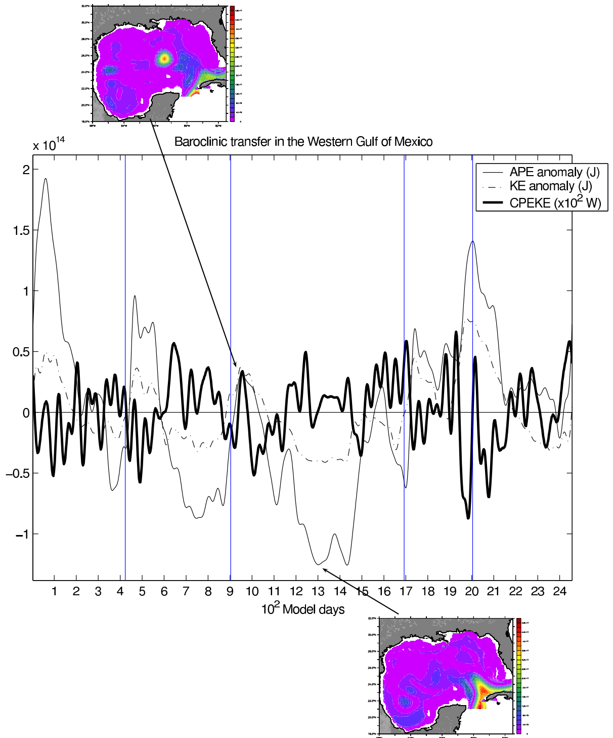
Figure 5.2: The baroclinic transfer in the western Gulf of Mexico. Vertical lines separate Loop Current cycles. Values are volume-integrated quantities. The upper Figure is a distribution of volume-integrated APE for a maximum level in potential energy, whereas the lower figure is a distribution for a minimum level.
