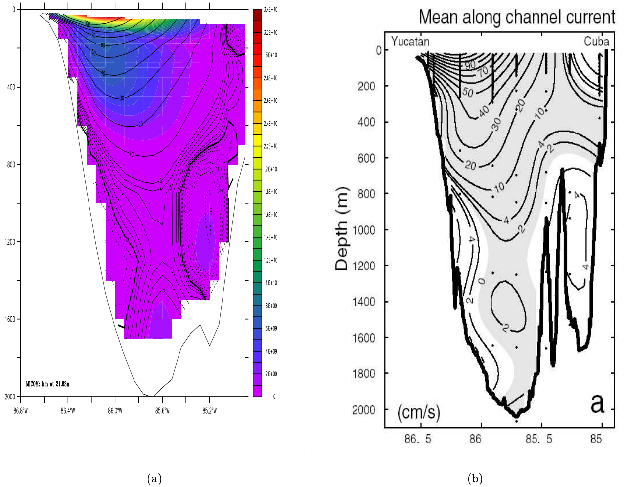
Figure 3.4: Time-averaged flow structure at the Yucatan Channel. (a) MICOM: solid(dashed) contours are for northward(southward) meridional velocities; color is kinetic energy of the mean flow (Joules). (b) Structure of the mean along-channel velocity field from observations (10-months time-average) [Sheinbaum et al., 2002].
