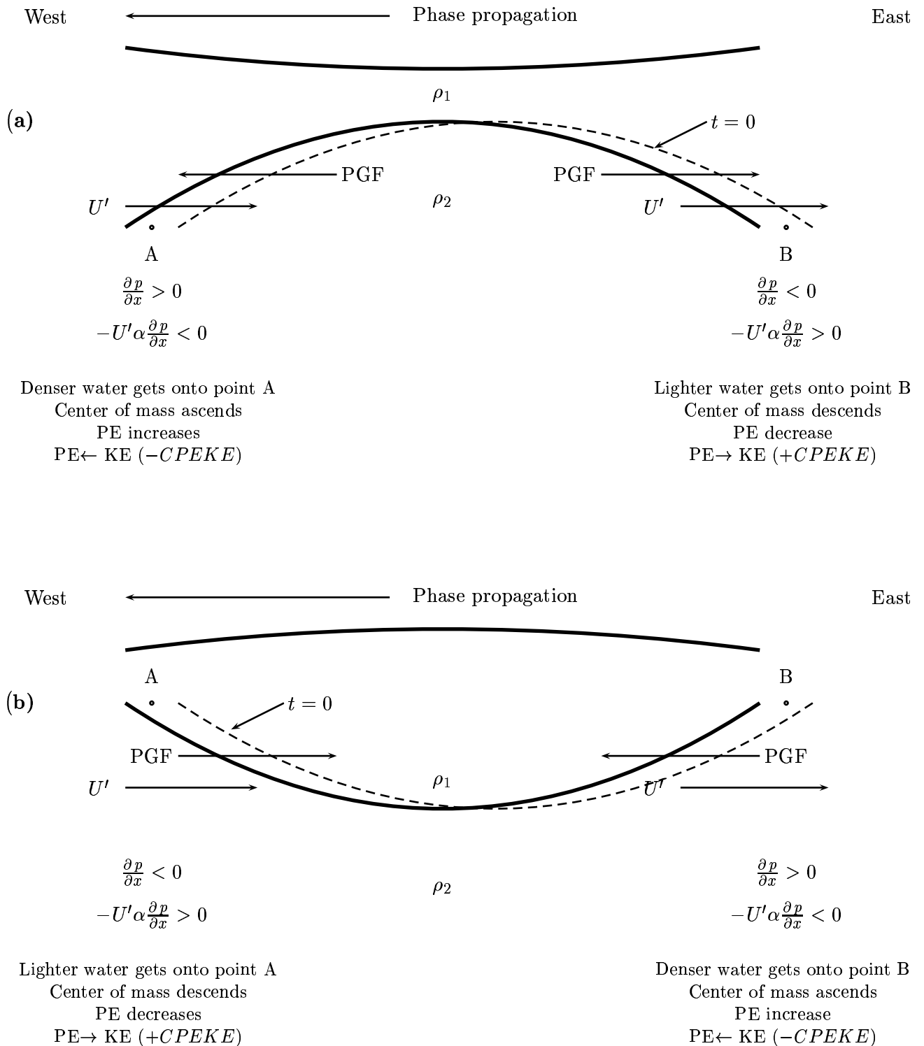
Figure 2.15: Mechanism of the baroclinic conversion, CPEKE , in isopycnal coordinates during the interaction of a fluctuating eastward flux with a westward propagating wave. (a) Cyclonic part of the wave (crest). (b) Anticyclonic part of the wave (trough).
