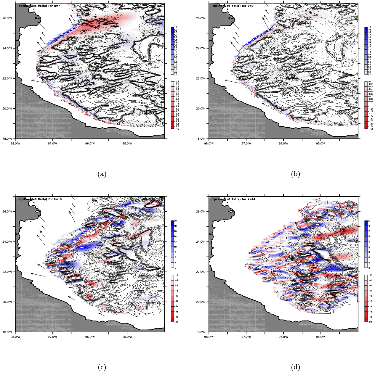
Figure 5.6: 7years-averaged CPEKM (color scale in 10^6 Watts) and Reynolds stress (contours) at the Western Boundary Current in the Mexican shelf. The arrows indicate the orientation of the local \beta -north. (a) Layer 7 ( \sim 300\text{m} depth), (b) layer 9 ( \sim 700\text{m} depth), (c) layer 13 ( \sim 1700\text{m} depth), and (d) layer 14 (below 2000m in average).
