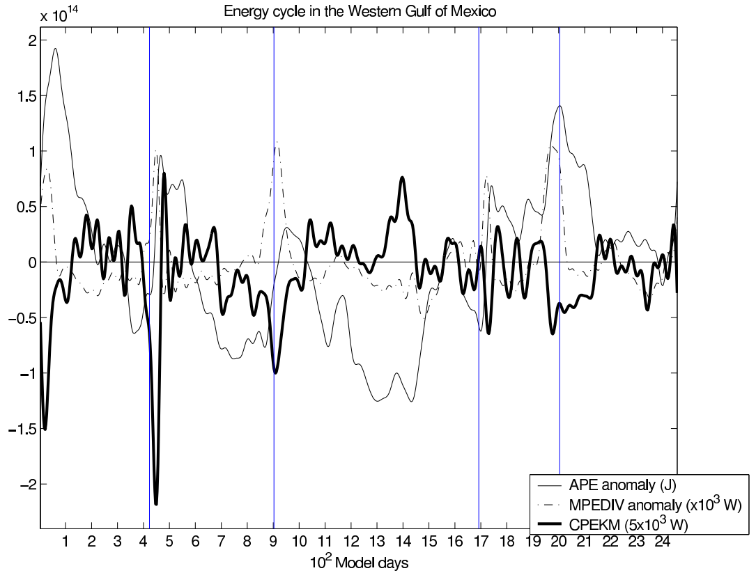
Figure 5.1: The energy cycle in the western Gulf of Mexico (to the west of 89W). Vertical lines separate Loop Current cycles. Values are volume-integrated quantities.
