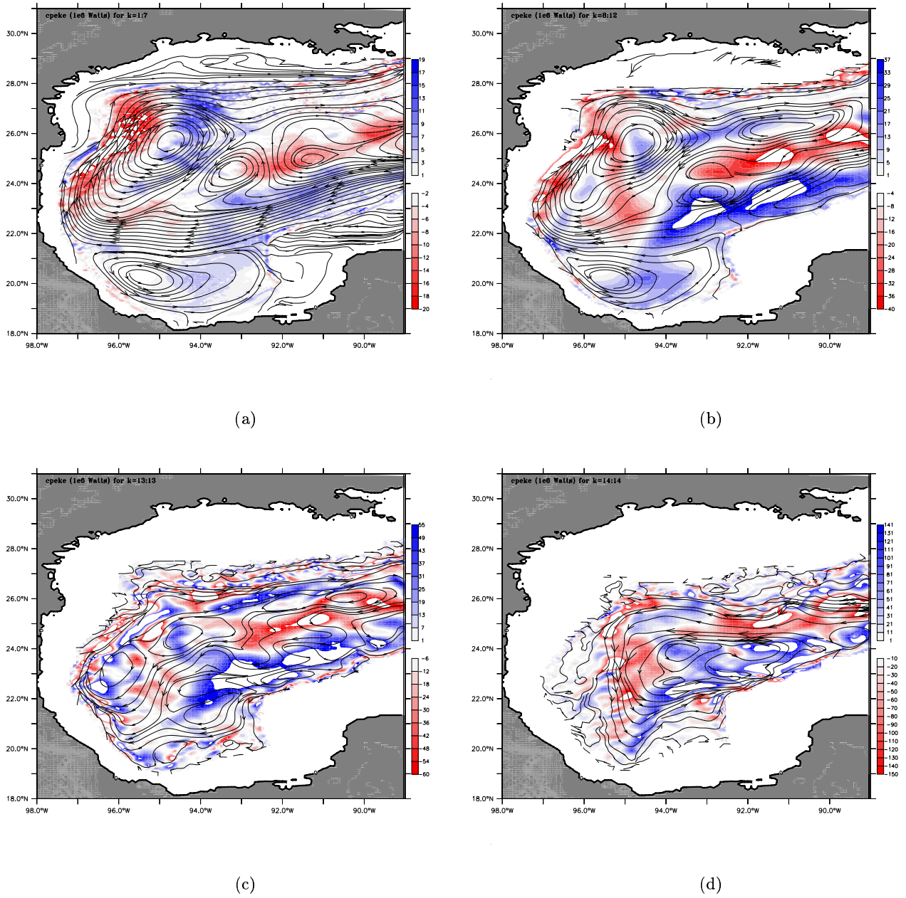
Figure 5.9: 7years-averaged CPEKE (color scale in 10^6 Watts) and flow lines at the western Gulf of Mexico. (a) Surface waters, (b) sub-surface waters, (c) intermediate waters, and (d) deep waters.
