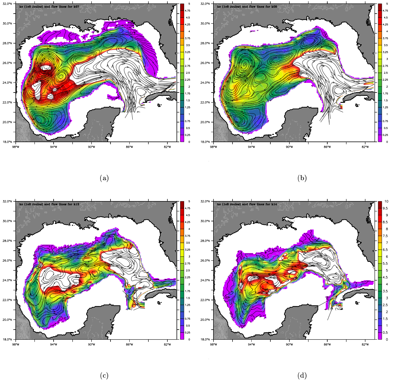
Figure 5.4: 7years-averaged, volume-integrated mean kinetic energy of the eddy flow, KE , at four model layers ( 10^8 Joules). (a) Layer 7 (~300m depth), (b) layer 9 (~700m depth), (c) layer 13 (~1700m depth), and (d) layer 14 (below 2000m in average).
