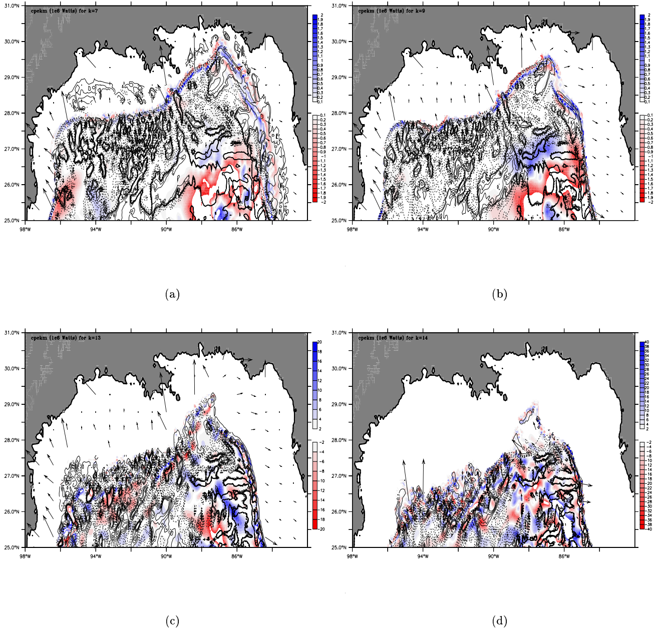
Figure 5.8: 7years-averaged CPEKM (color scale in 10^6 Watts) and Reynolds stress (contours) at the Northern Gulf of Mexico. The arrows indicate the orientation of the local \beta -north. (a) Layer 7 (~300m depth), (b) layer 9 (~700m depth), (c) layer 13 (~1700m depth), and (d) layer 14 (below 2000m in average).
