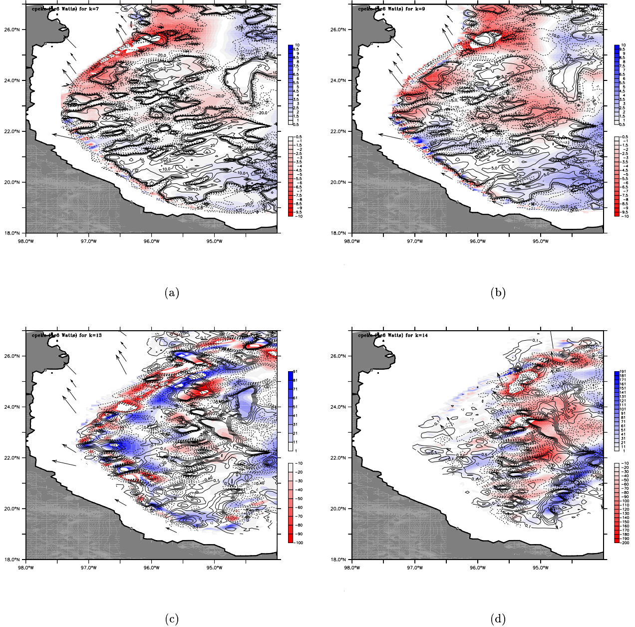
Figure 5.5: 7years-averaged CPEKE (color scale in 10^6 Watts) and Reynolds stress (contours) at the Western Boundary Current in the Mexican shelf. The arrows indicate the orientation of the local \beta -north. (a) Layer 7 ( \sim 300 m depth), (b) layer 9 ( \sim 700 m depth), (c) layer 13 ( \sim 1700 m depth), and (d) layer 14 (below 2000m in average).
