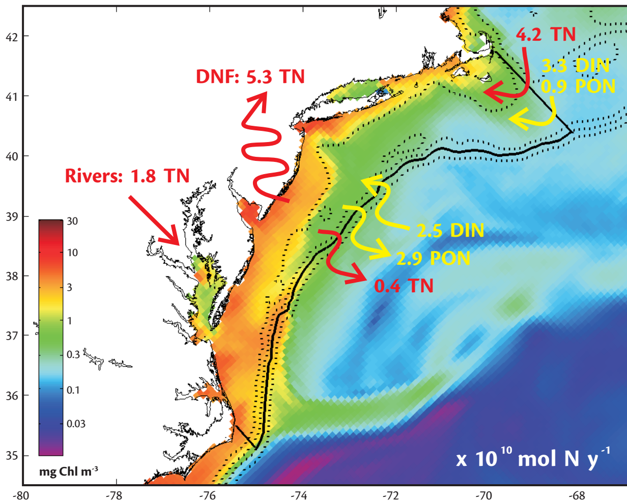
Figure 9. Model predicted mean surface chlorophyll for July 1994 in the Middle Atlantic Bight (MAB) overlain by a model-derived nitrogen budget for the MAB shelf region. An annual mean nitrogen budget for the MAB shelf region (indicated by the solid black lines) was derived by diagnosing the fluxes of total nitrogen (TN, red numbers and arrows), dissolved inorganic nitrogen (DIN, yellow) and particulate organic nitrogen (PON, yellow) across two cross-shelf transects at Cape Cod and Cape Hatteras and across the 200 m isobath (the 40, 100, 200, and 500 m isobaths are indicated by dotted black lines) in addition to the annual river input and the denitrification (DNF) loss.
