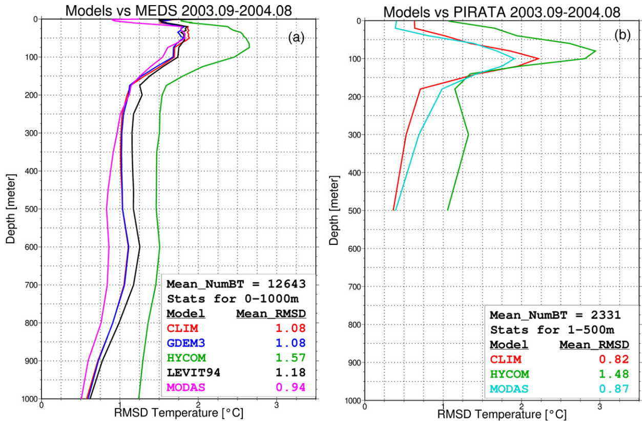
Fig. 12. (a) Statistics for September 2003 through August 2004 between the 1/12° HYCOM system and available Marine Environmental Data Service (MEDS) profile observations. The RMS difference between the MEDS data and different climatologies, MODAS climatology (CLIM), MODAS synthetics (MODAS), Levitus et al. (1994), and the Generalized Digital Environmental Model (GDEM3) is also shown. (b) Statistics for September 2003 through August 2004 between the 1/12° HYCOM system and available PIRATA profile observations. The RMS between the PIRATA data and the MODAS climatology (CLIM) and MODAS synthetics (MODAS) is also shown.
