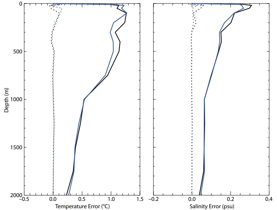
Figure 2. In situ profile innovation statistics for FOAM (Forecast Ocean Assimilation Model) global 1/4^\circ (black) and regional 1/12^\circ (blue) models in the North Atlantic computed over one year (from April 1, 2005, to March 31, 2006). Dark lines = RMS error. Dotted lines = bias (left is temperature, right is salinity).
