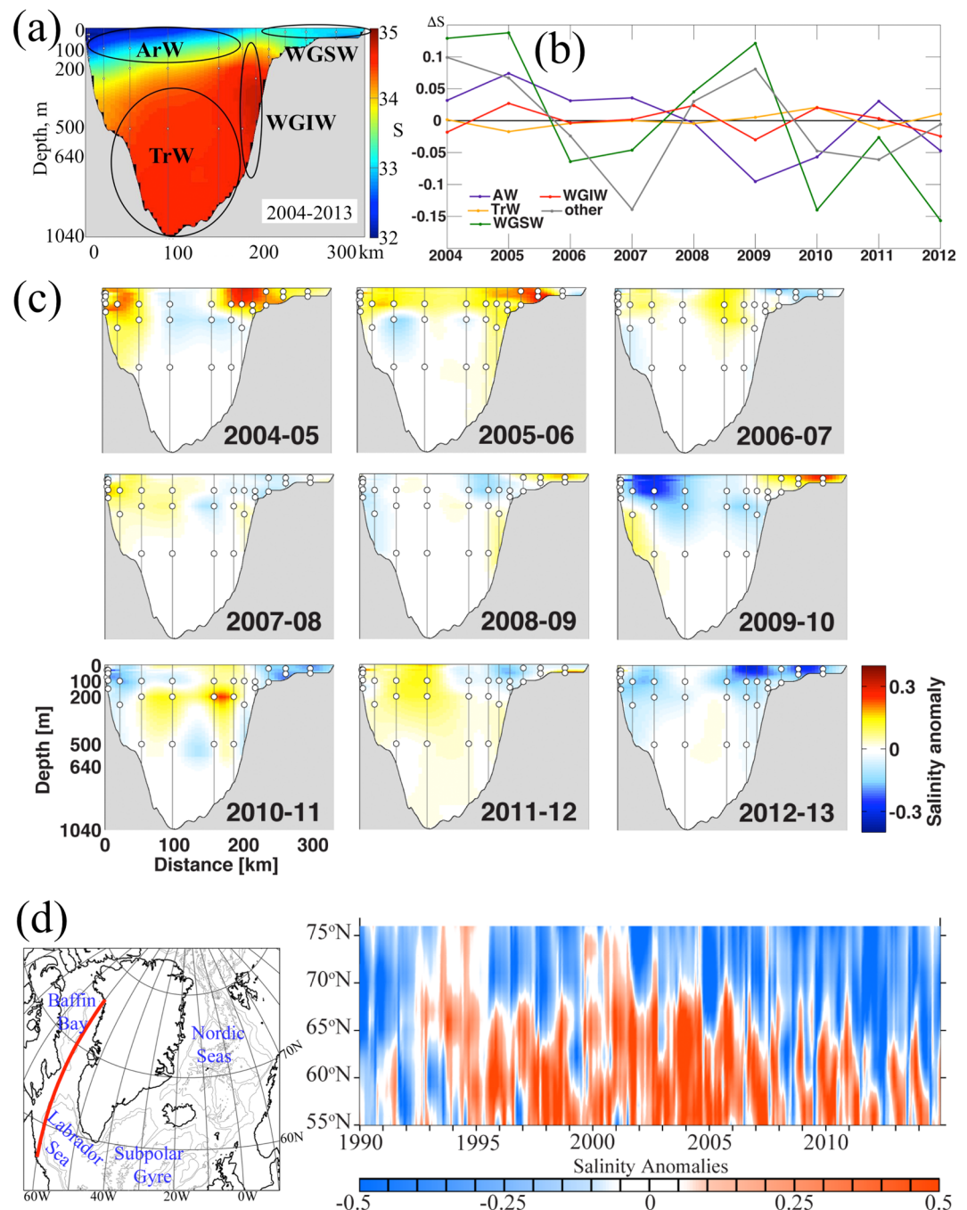
Figure 3. Mean salinity and salinity anomalies derived from the observational program in Davis Strait data between 2004 and 2013 (the location of the moored array is shown in Figure 1). (a) Mean salinity. The major water masses are indicated: ArW – Arctic Water, TrW – Transitional Water, WGIW – West Greenland Irminger Water, WGSW – West Greenland Shelf Water. (b) Annual salinity anomalies ( \Delta S ) relative to the 2004–2013 mean for the individual water masses. The other water mass refers to the near surface water that is too warm to be classified as ArW or is near surface water along the West Greenland slope right at the shelf that is too salty to be WGSW and too fresh to be WGIW. (c) Annual salinity anomalies relative to the 2003–2013 mean. (d) Time versus latitude diagram showing salinity anomalies along the section shown with the red line on the map to the left for the time period from 1990 to 2014 relative to the 1960–1990 monthly climatology. Salinity climatology and anomalies are derived from the Met Office Hadley Centre subsurface ocean salinity data set (EN.4.1.1).
