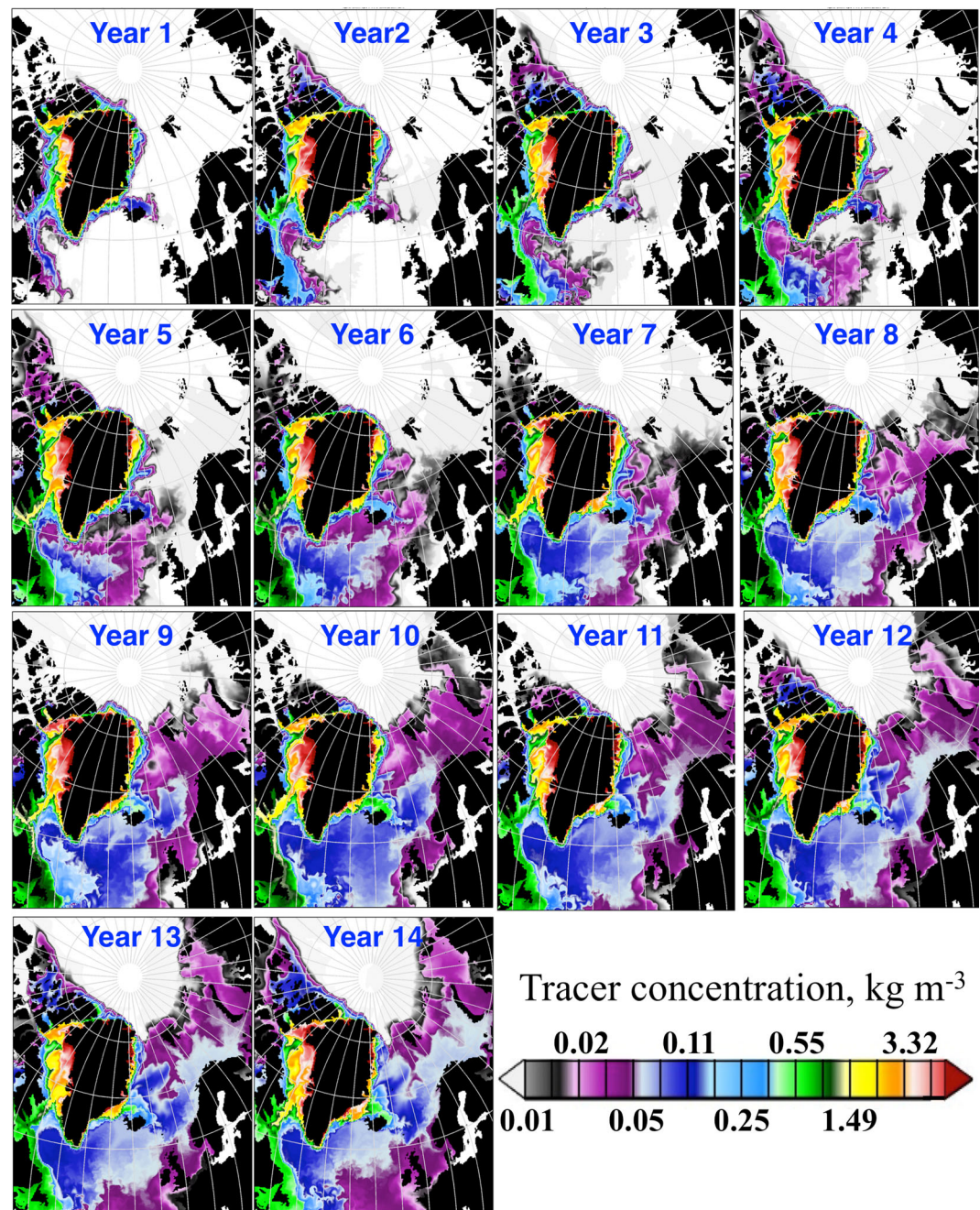
Figure 6. Five-day mean tracer concentration in the surface model layer (~1 m) for output including 17 December for every model year from NEMO-LIM2. The concentration is on the natural-log scale ( \text{kg m}^{-3} ).
