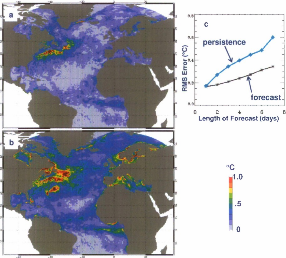
Figure 7: Spatial distribution of rms error for (a) the 1-day and (b) the 7-day 1/12° operational Mercator Ocean SST forecasts. The time evolution of the SST error growth in comparison to persistence is shown in (c). The statistics were computed from the forecasts over the 4-month time period June-Sept. 2008.
