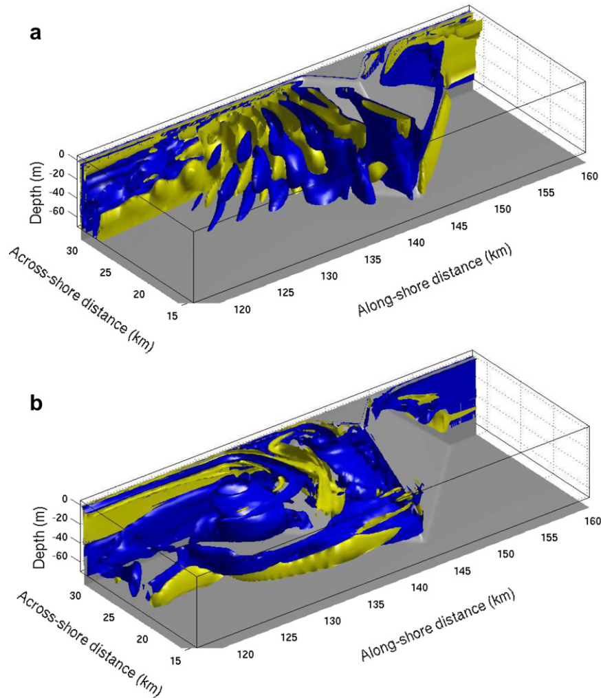
Fig. 2. Three-dimensional views of relative vorticity iso-surfaces in the vicinity of the cape. Negative values are shown in blue, while positive values are in yellow. (a) Exp. 16: a typical example of fully attached regime, when no separation occurs and lee waves are evident in the lee of the obstacle. (b) Exp. 21: an example of eddy-shedding regime. The flow is almost two-dimensional and flow separation is observed behind the cape.
