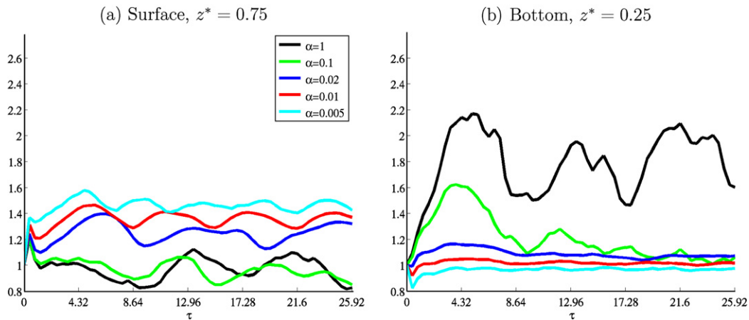
Fig. 7. The ratio KE/KE_0 in time for varying obstacle slopes \alpha . The Burger number is Bu = 1.00 in all the considered simulations.
