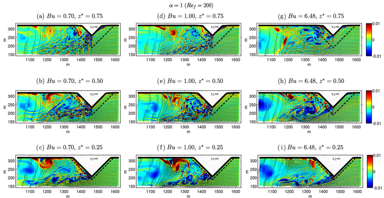
Fig. 4. As in Fig. 3 but for different Bu .
