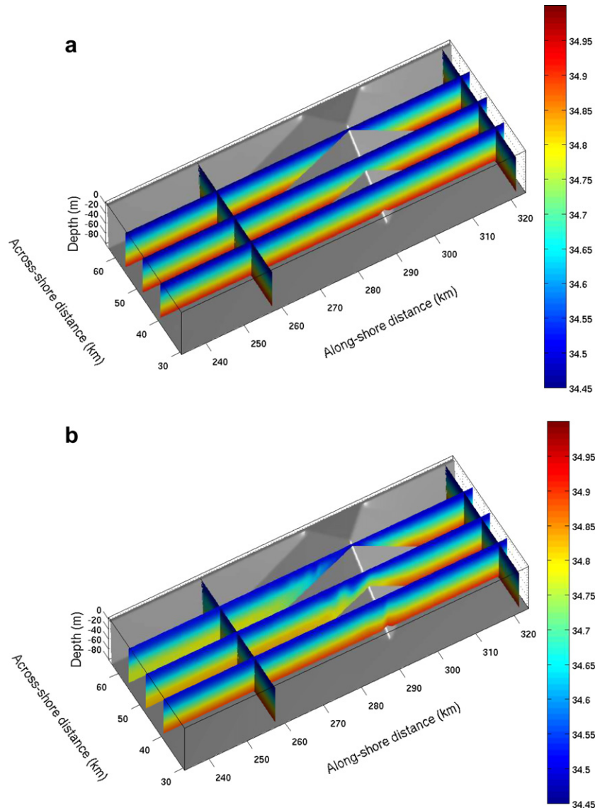
Fig. 15. Three-dimensional close up of the salinity field at different times for the case when Bu = 0.05 and \alpha = 0.005 . (a) \tau = 0 ; (b) \tau = 9.936 .
