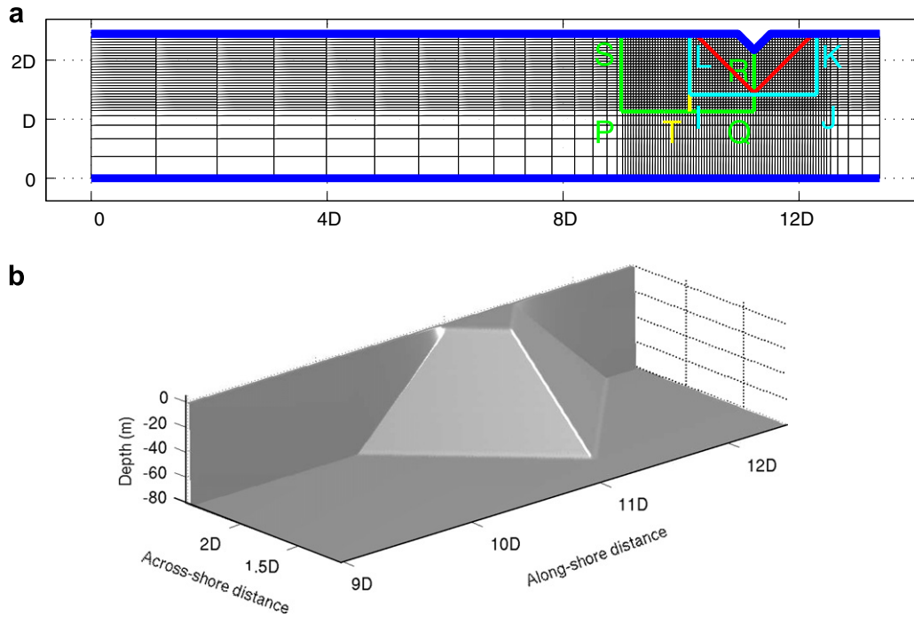
Fig. 1. Numerical setup expressed in terms of D . D is defined as the across-shore horizontal dimension of the obstacle at the bottom. (a) Plan view of the horizontal grid. For clarity, every third grid-point is shown in the picture. The northern and southern boundaries are closed (blue thick line) while the eastern and western are open. The red line indicates where the slope terminates. The areas PTLs (yellow), IJKL (cyan) and PQRS (green) are functional to later calculations of the vertical velocity, the kinetic energy and the form drag, respectively. (b) Three-dimensional shape of the cape.
