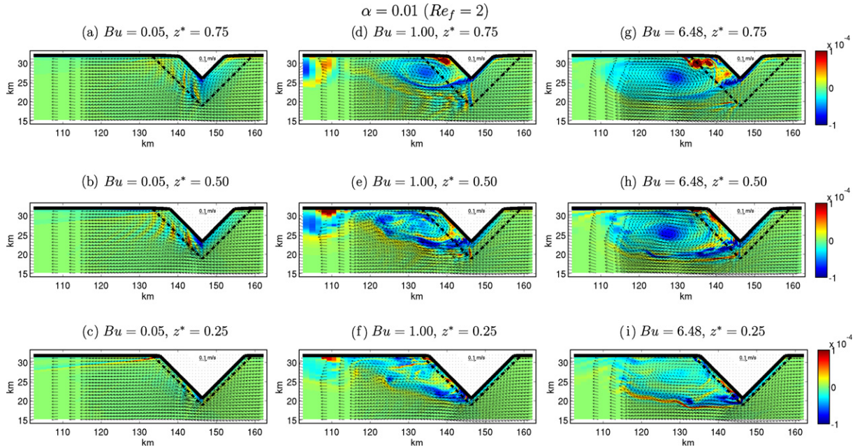
Fig. 6. As in Fig. 3 but for \alpha = 0.01 .
