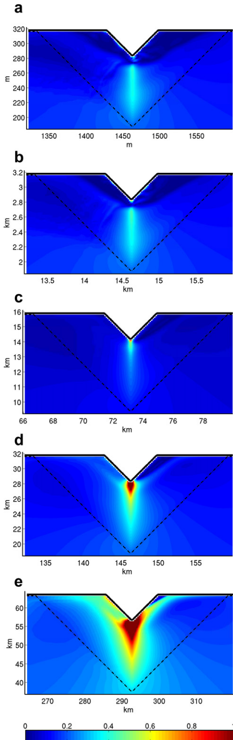
Fig. 16. Plan views of the local internal Froude numbers for the simulations with Bu = 0.05 and different \alpha . In all the plots \tau = 9.936 and the dotted line indicates where the slope ends. (a) \alpha = 1 ; (b) \alpha = 0.1 ; (c) \alpha = 0.02 ; (d) \alpha = 0.01 ; (e) \alpha = 0.005 .
