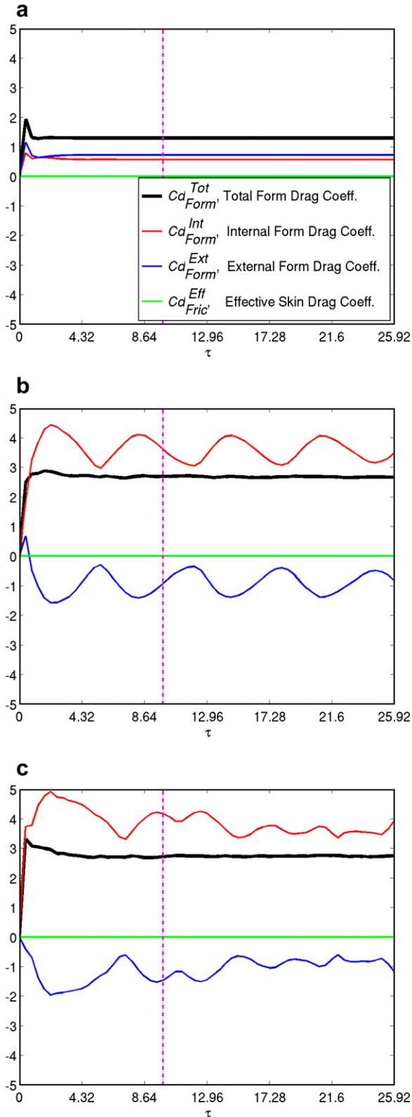
Fig. 11. Drag coefficients in time for the \alpha = 0.01 simulations. The magenta dot-dashed vertical line indicates the specific time for Fig. 13. (a) Bu = 0.05 ; (b) Bu = 1.00 ; (c) Bu = 6.48 .
