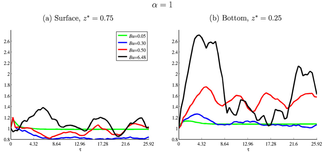
Fig. 5. The ratio KE/KE_0 in time for varying Burger numbers Bu . The obstacle slope is \alpha = 1 in all the considered simulations.
