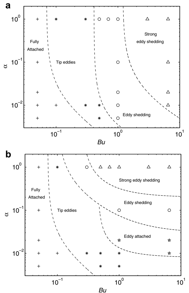
Fig. 8. Different regimes varying Bu and the slope \alpha for (a) surface and (b) bottom. Note that both axes are logarithmic. The regimes are: fully attached (+), tip eddies (*), eddy-attached (☆), eddy-shedding (o) and strong eddy-shedding ( \Delta ). The dashed lines are the approximate divisions between the regimes. (a) Surface; (b) bottom.
