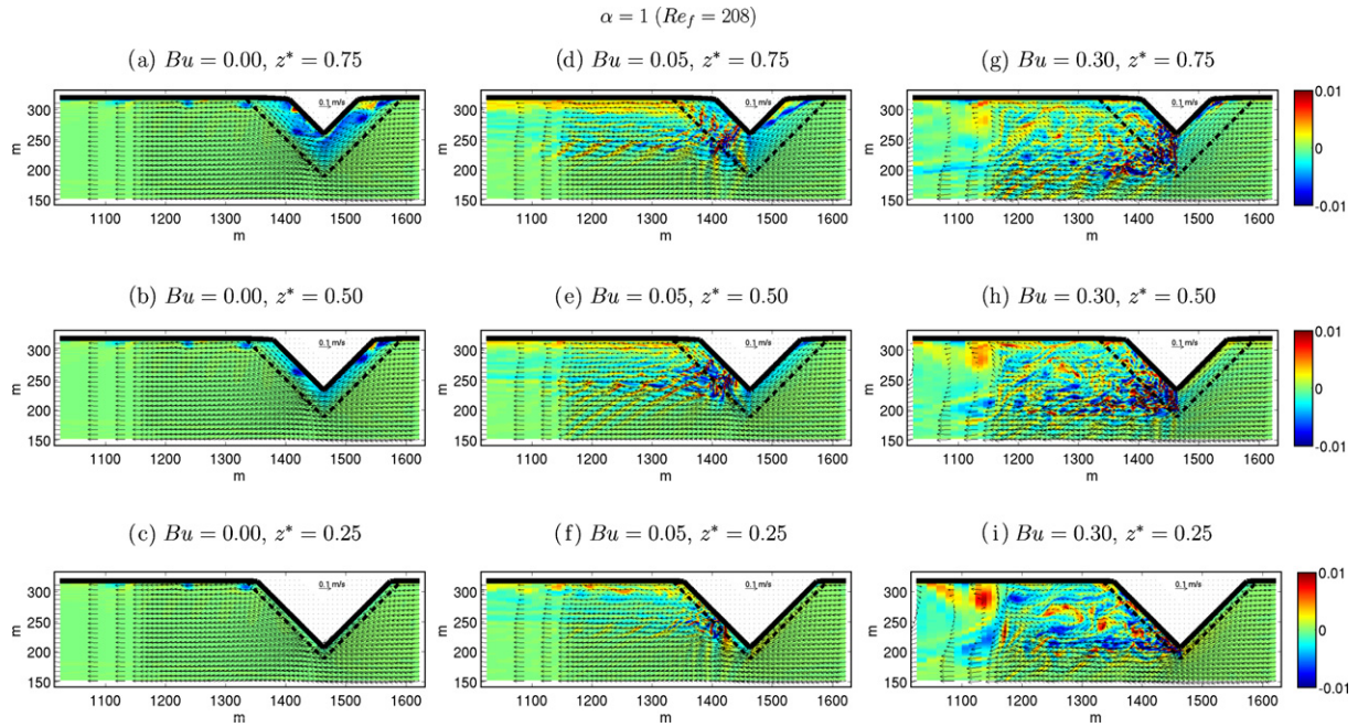
Fig. 3. Close up of relative vorticity ( s^{-1} ) and velocity vectors at three different levels of the water column ( z^* = z/H ) after \tau = 9.936 for the \alpha = 1 simulations. The black dash-dotted line indicates where the slope terminates.
