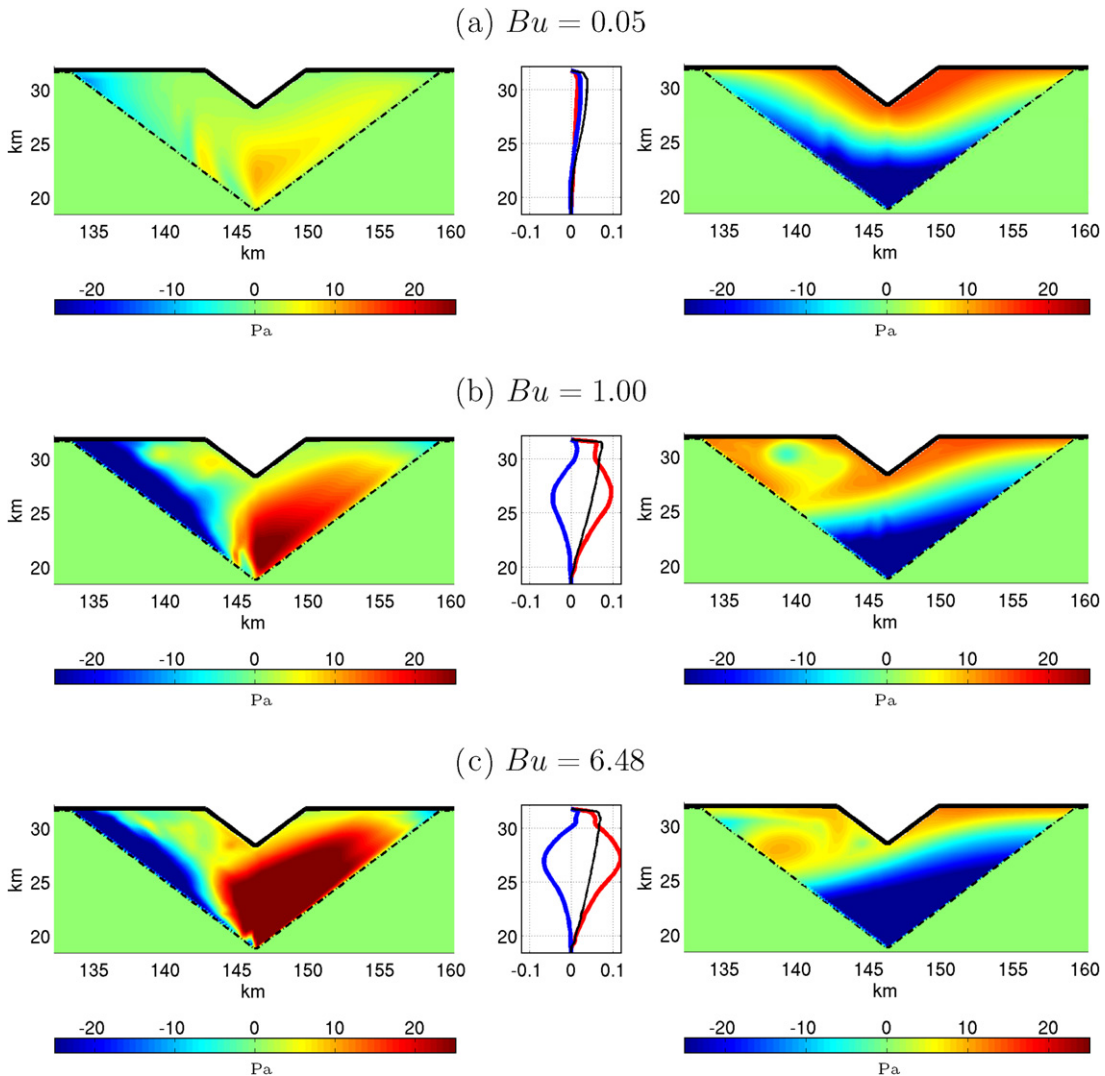
Fig. 13. Left panels: Plan view of the quantity I . Center panels: The non-dimensional along-shore integrated quantities S_T (black thin line), S_I (red line) and S_E (blue line) as a function of the across-shore direction. Right panels: plan view of the quantity E . In all the plots \alpha = 0.01 , \tau = 9.936 and the dash-dotted line indicates where the slope ends.
