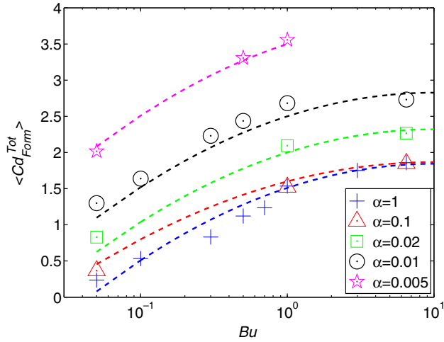
Fig. 12. Total drag coefficients as a function of Bu and \alpha . Symbols refer to experiments and dashed lines are from Eq. (2). Note that the x -axis is logarithmic.
