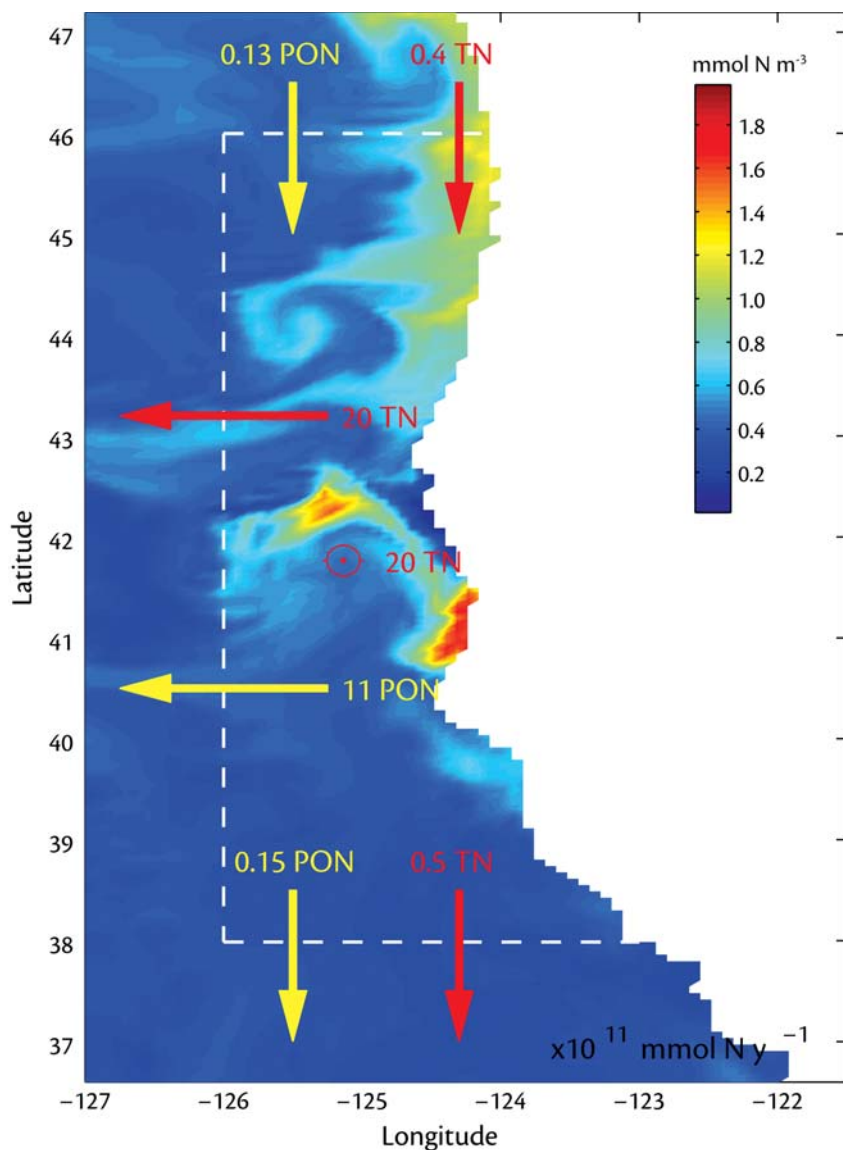
Figure 10. Model-predicted mean surface chlorophyll for July in the California Current System overlain by a model-derived annual mean nitrogen budget within a near-surface box delimited from below by the \sigma_{25} isopycnal and horizontally as indicated by the white dashed lines. Shown in the figure are transports of total nitrogen (TN) and particulate organic nitrogen (PON). Note that more than a half of the upwelled inorganic nitrogen is exported offshore as PON, mainly via filaments of the California Current.
