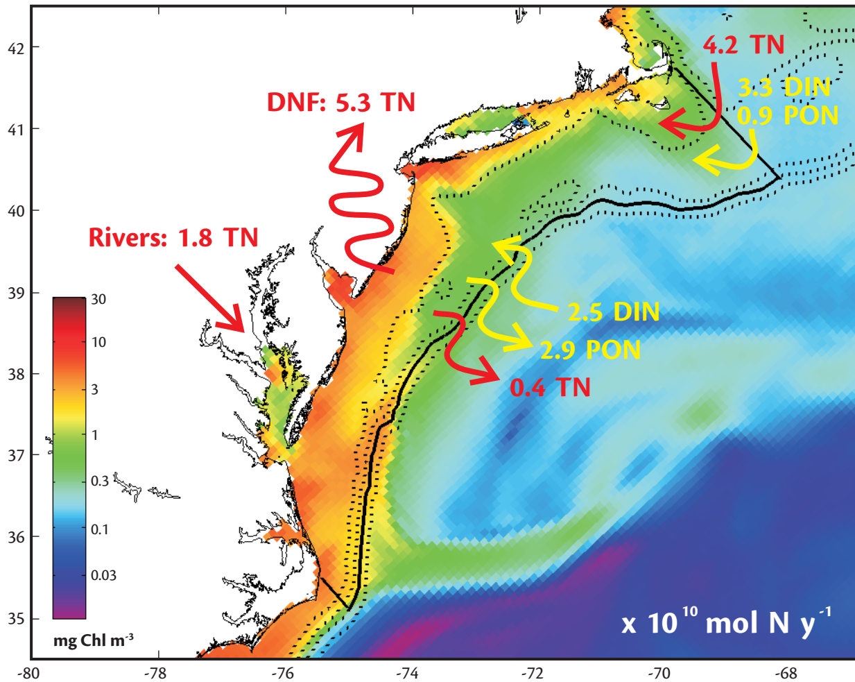
Figure 9. Model predicted mean surface chlorophyll for July 1994 in the Middle Atlantic Bight (MAB) overlain by a model-derived nitrogen budget for the MAB shelf region. An annual mean nitrogen budget for the MAB shelf region (indicated by the solid black lines) was derived by diagnosing the fluxes of total nitrogen (TN, red numbers and arrows), dissolved inorganic nitrogen (DIN, yellow) and particulate organic nitrogen (PON, yellow) across two cross-shelf transects at Cape Cod and Cape Hatteras and across the 200 m isobath (the 40, 100, 200, and 500 m isobaths are indicated by dotted black lines) in addition to the annual river input and the denitrification (DNF) loss.
