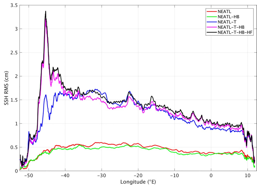
Figure 3. Standard deviation of the high-frequency steric sea surface height (in cm) variability in the equatorial Atlantic (averaged between 5°S and 5°N) in five 1/50° Atlantic simulations that are shown in Figure 2: (a) NEATL, (b) NEATL-HB, (c) NEATL-T, (d) NEATL-T-HB, and (e) NEATL-T-HB-HF.
