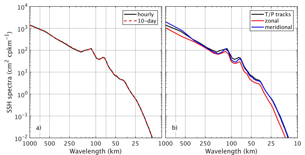
Figure 12. Impact of temporal/spatial sampling on sea surface height wavenumber calculation: panel (a) shows the spectra calculated from tracks that are sampled every hour vs. every 10 days; panel (b) shows the spectra calculated from Topex/Poseidon tracks vs. from zonal and meridional tracks with full model resolution.
