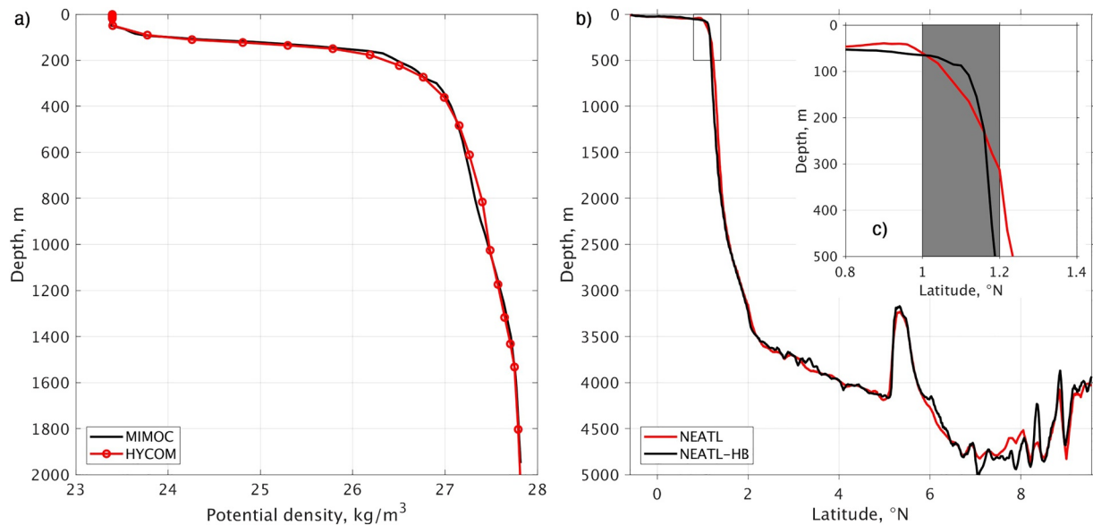
Figure 6. (a) density profile off the Amazon shelf in 1/50^\circ Hybrid Coordinate Ocean Model simulation NEATL-T-HB-HF and in ocean climatology MIMOC (Schmidt et al., 2013); (b) The model bathymetry along a north-northeastward section from the Amazon shelf to the open ocean (dashed line in Figures 4a and 4b) in two 1/50^\circ simulations with and without high-resolution bathymetry variability; the insert panel (c) shows the bathymetry zoomed near the shelf break, as denoted by the small rectangle in panel (b).
