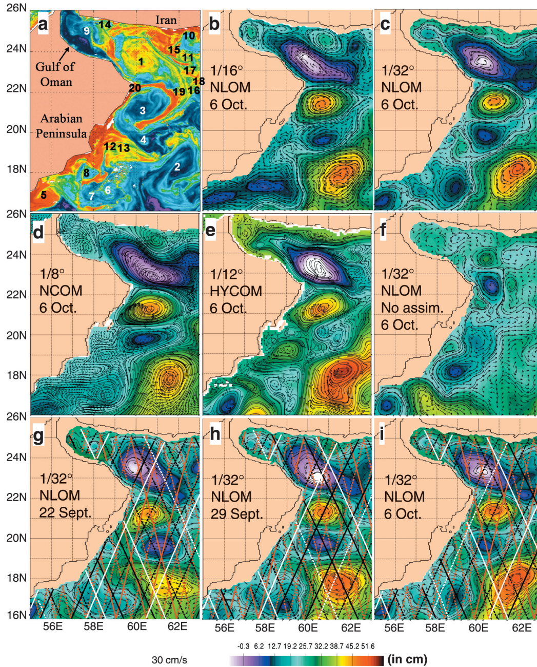
Plate 2. A comparison of eddies and currents seen in (a) chlorophyll concentration from SeaWiFS (October 2–6, 2002, latest cloud-free pixel composite with most data from October 6) with (b–e) data-assimilative model nowcast SSH and currents on October 6, 2002 from (b) 1/16° global NLOM, (c) 1/32° global NLOM, (d) 1/8° global NCOM, and (e) 1/12° global HYCOM. (f) same as (c) but without ocean data assimilation. In (a), eddies with clearly-defined eddy centers are numbered in order of decreasing size for use in Table 2. The color of the number varies only for visual clarity. 1/32° NLOM SSH and currents for (g) September 22, 2002; (h) September 29, 2002; (i) October 6, 2002 [same as (c)] with the most recent week of observed altimeter tracks overlaid as solid lines and the remaining tracks as dashed lines, red for ERS-2, black for GFO, and white for Jason-1. At the time, Jason-1 data were not available in real time at NAVOCEANO and thus not assimilated by the operational 1/16° NLOM system which provided the results used in (b). Note that a few of the smallest eddies are not visible due to limitations of the small plots or because they were slightly east of 63°E in a model result. NLOM results are adapted from Shriver et al. [2007].
