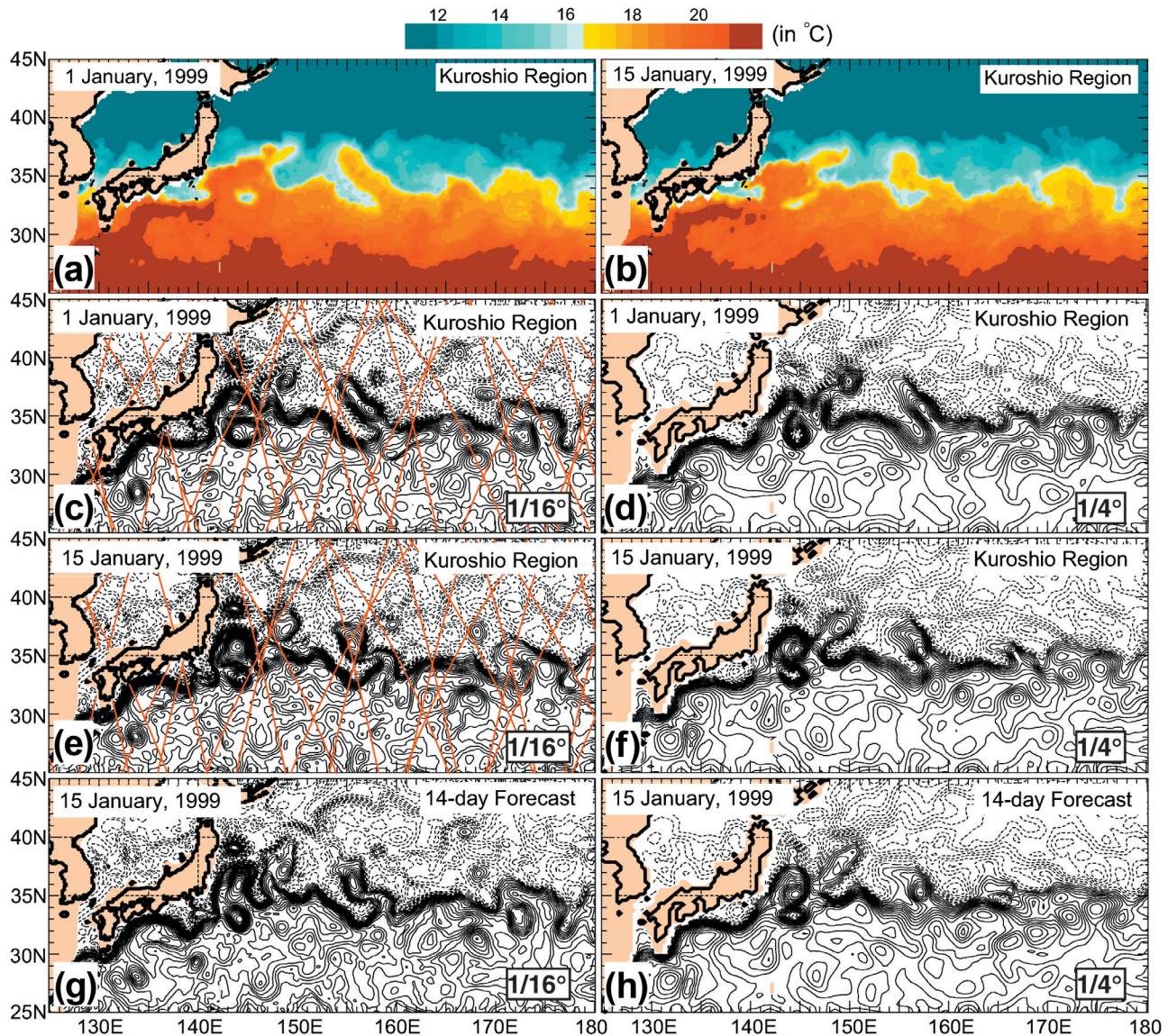
Plate 1. Kuroshio region (a, b) NAVOCEANO operational 1/8^\circ MODAS SST analyses for (a) January 1, 1999 and (b) January 15, 1999 with the color bar ( 0.5^\circ\text{C} interval) designed to highlight the Kuroshio pathway, (c-f) SSH analyses ( 5\text{-cm} interval) with assimilation of altimeter track data from TOPEX/Poseidon and ERS-2 using the model forecast as the first guess from (c, e) 1/16^\circ Pacific NLOM and (d, f) 1/4^\circ global NLOM for (c, d) January 1, 1999 and (e, f) January 15, 1999. The altimeter tracks assimilated on the date given (using a 3-day data window) are overlaid in red on (c, e). (g, h) The 14-day forecast SSH from (g) 1/16^\circ Pacific NLOM and (h) 1/4^\circ global NLOM. Adapted from Hurlburt et al. [2000].
