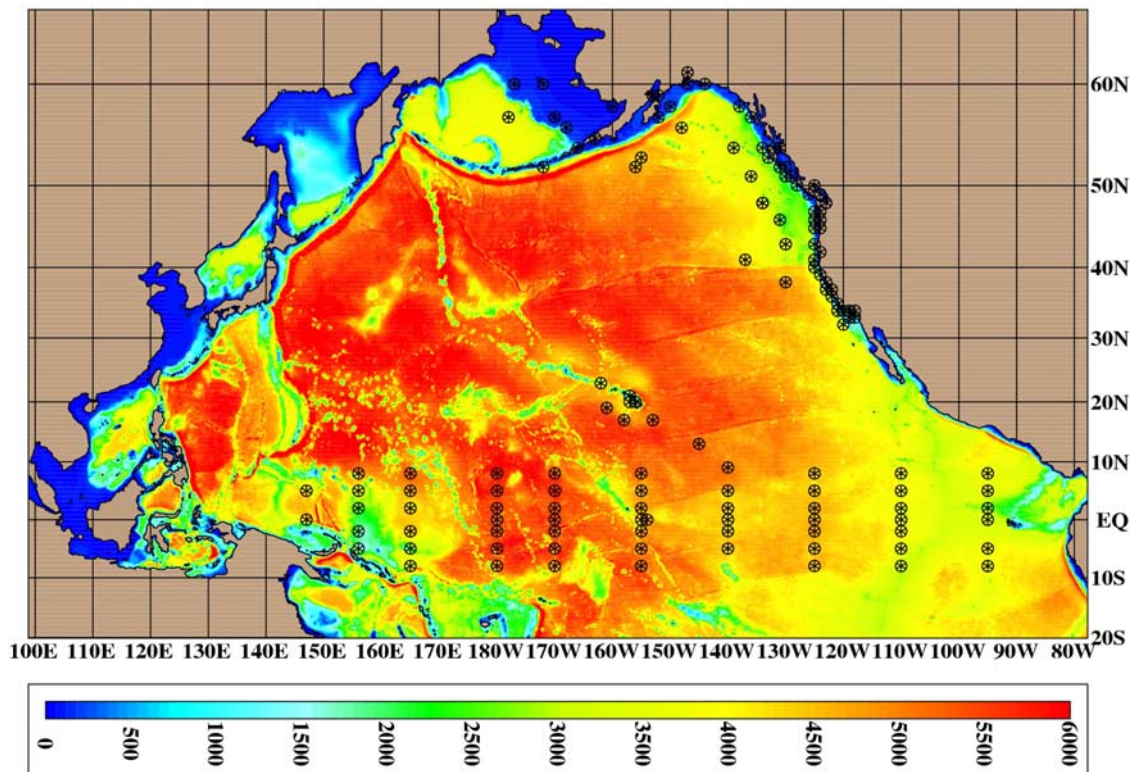
Figure 1. Locations of 135 buoys superimposed on the bottom topography of the Pacific HYCOM domain. The model land/sea boundary is the 10-m isobath. The TAO array has been reporting high temporal resolution (e.g., hourly and daily) SST time series over the equatorial Pacific since 1986. Hourly SST time series from NDBC have been available over coastal and open-ocean locations since at least the 1970s. The Environmental Monitoring Division of Canada network of moored buoys has been reporting hourly SST time series along the coasts of Canada since the 1990s. Most of the reliable data have been collected since 1990. Thus we use buoy SST time series observed during 1990–2003.
