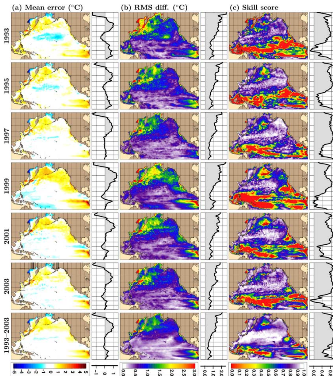
Figure 3. Annual maps of (a) mean error (ME), (b) RMS SST difference, and (c) SST skill score (SS) between HYCOM and MODAS given for every other year from 1993 through 2003. Statistical metrics are described in section 4.1. Statistics over all years (1993–2003) are shown in the last row. Zonal averages are provided next to each panel.
