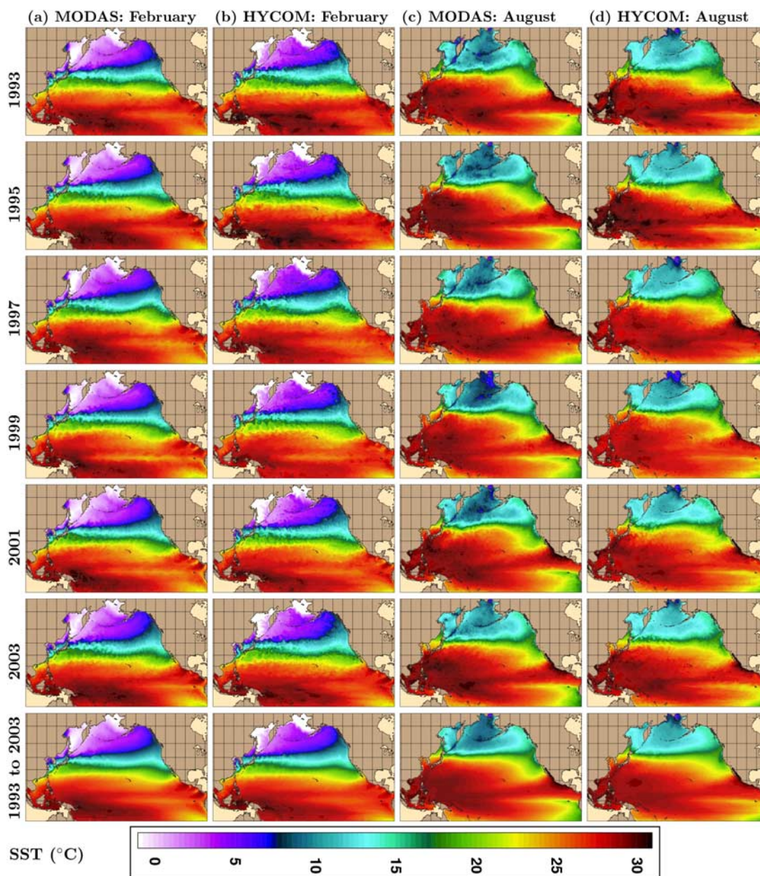
Figure 2. Monthly mean MODAS and HYCOM SST over the North Pacific in February and August. They are shown every other year during 1993–2003, along with mean SST over all years (1993–2003). HYCOM does not assimilate any ocean data or relax to any SST data, including MODAS.
