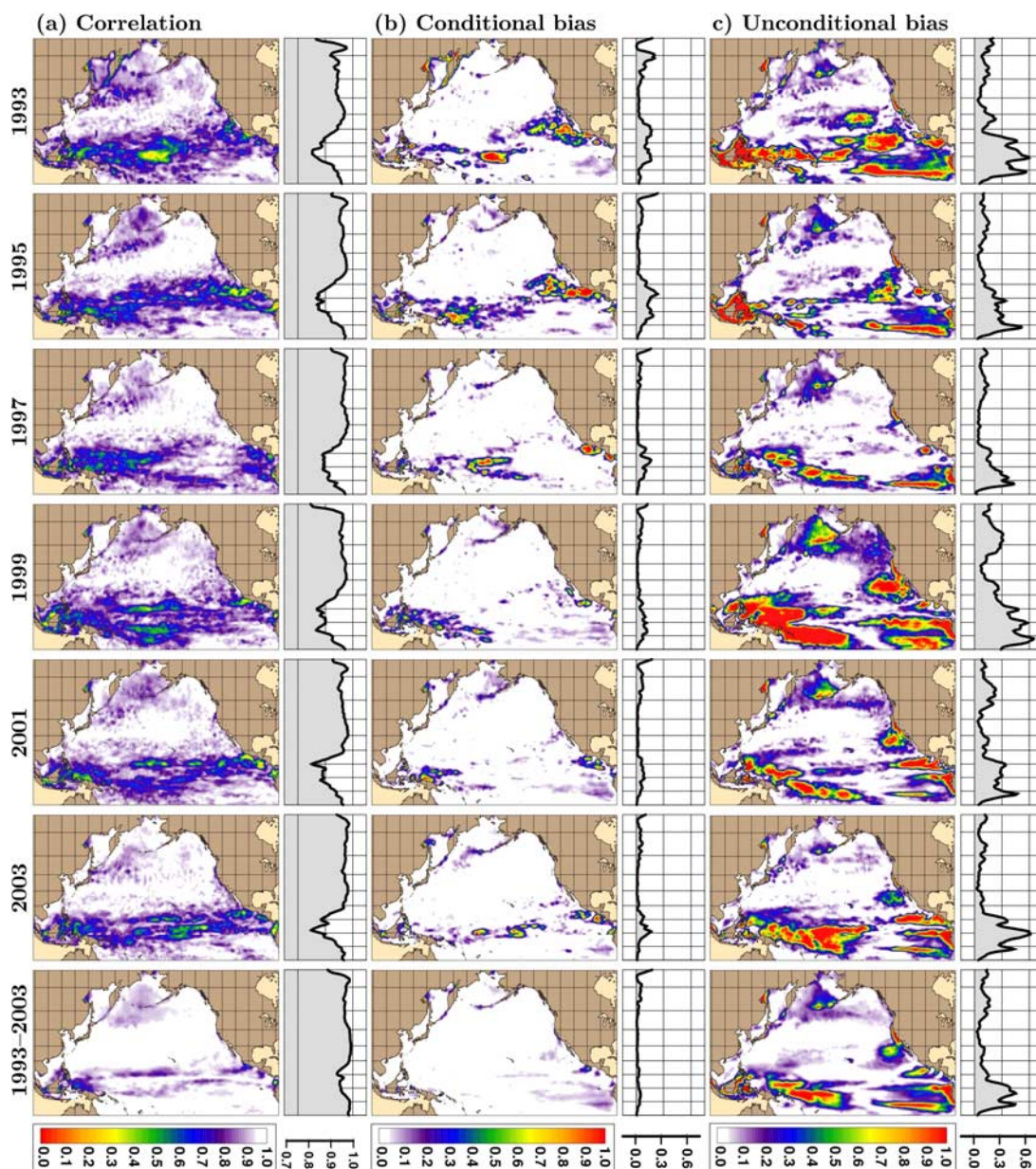
Figure 4. Same as Figure 3 but for (a) correlation coefficient ( R ), (b) conditional B_{\text{cond}} , and (c) unconditional B_{\text{uncond}} biases between HYCOM and MODAS SST. The white color represents R values of >0.95 and B_{\text{cond}} or B_{\text{uncond}} of <0.05 .
