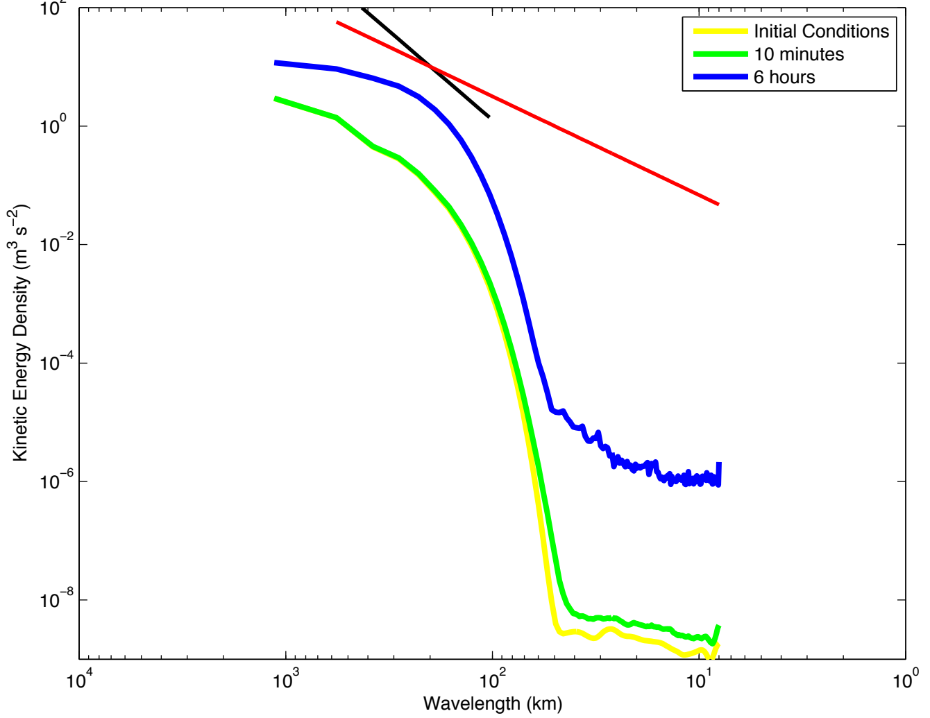
ng03 vortex (newer version) with NO dissipation and NO advection
