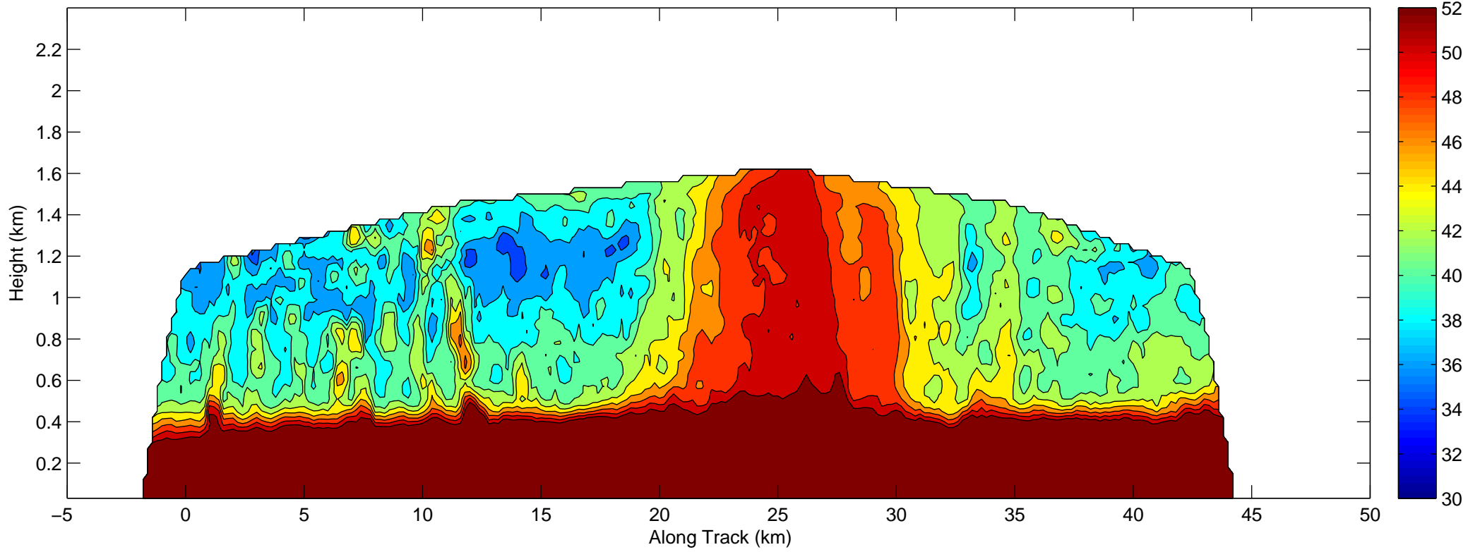
C band reflectivity cross section (1 km left of nadir)--Hurricane Isabel
