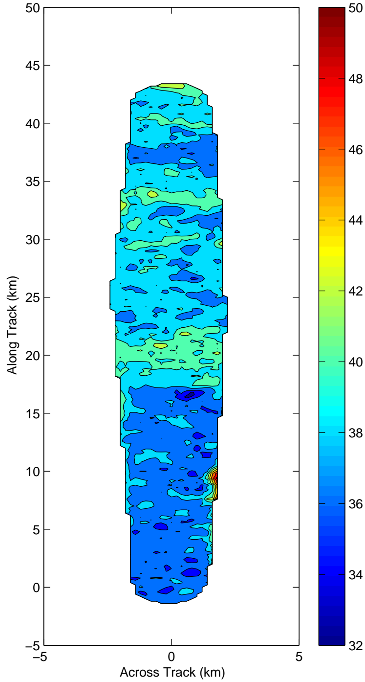
Ku band reflectivity at 630 meters height--Hurricane Isabel
