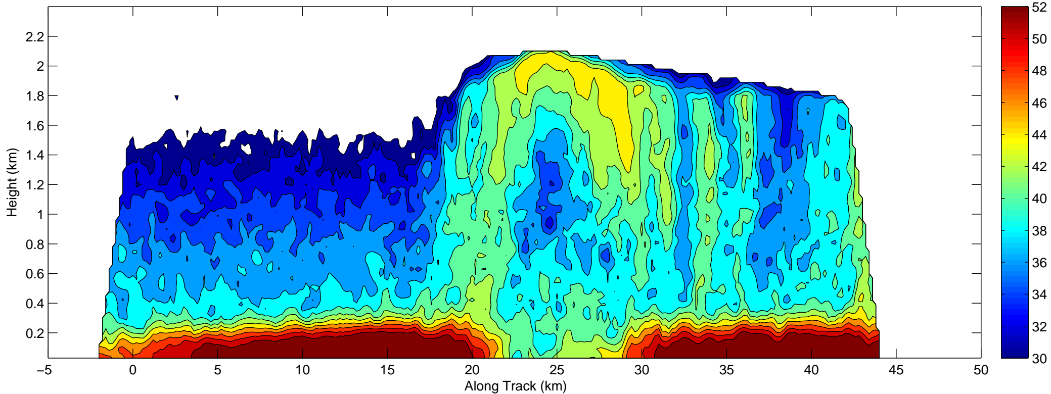
Ku band reflectivity cross section along aircraft track--Hurricane Isabel
