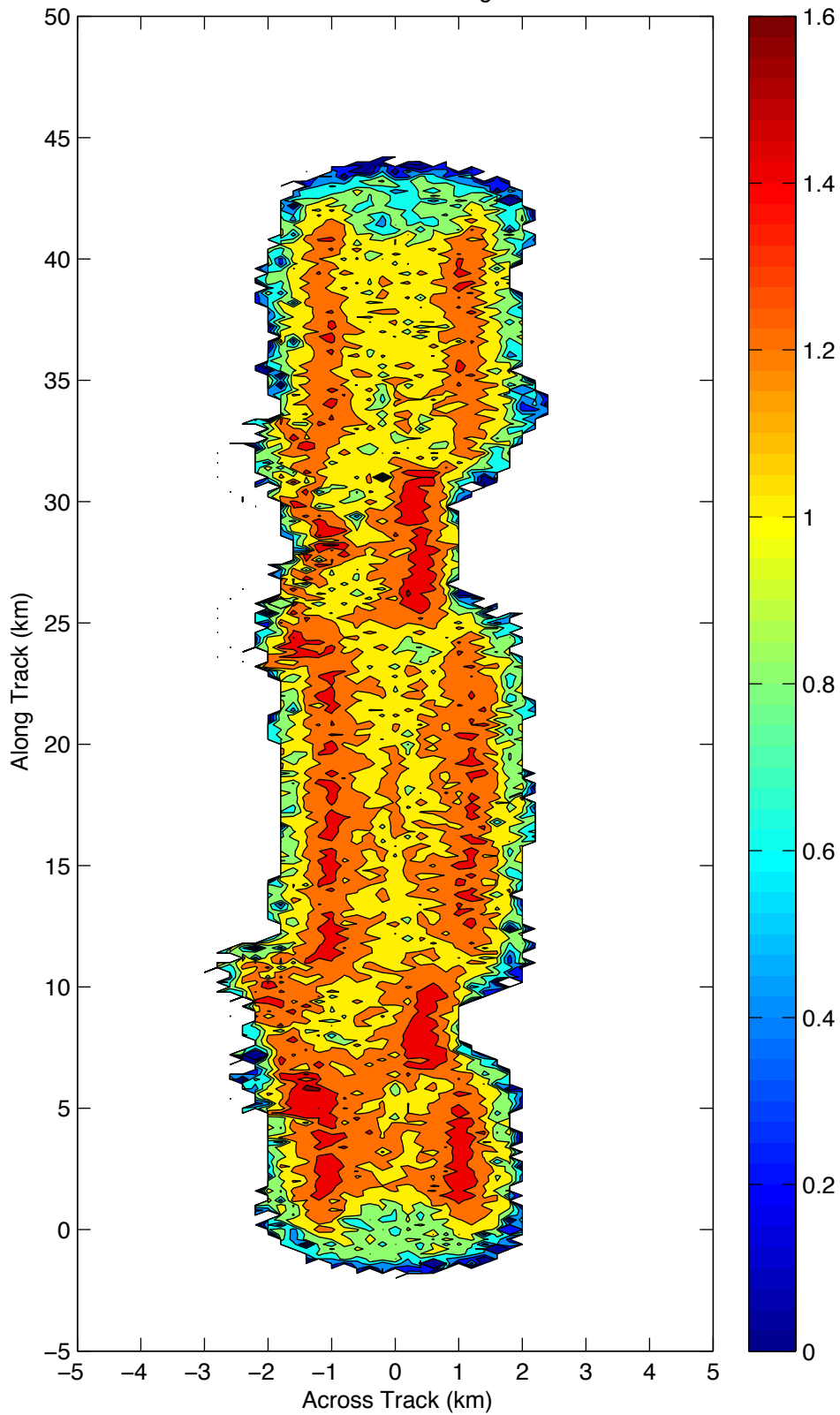
Number of pulses (log scale) in 200 m x 200 m x 30 m grid for all 4 beams at C Band slice at 0.50 km height
