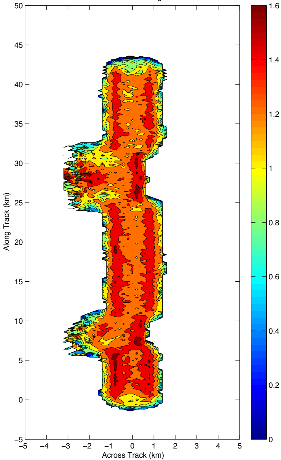
Number of pulses (log scale) in 200 m x 200 m x 30 m grid for all 4 beams at C Band slice at 1.0 km height
