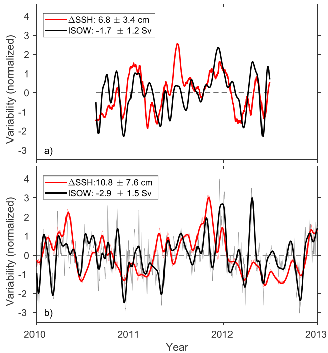
Figure 9. (a) Variability of the observed ISOW transport (low-passed by third-order, Butterworth filter) and the sea surface height (SSH) difference across the CGFZ between 52.125 and 53.125°N along 35.25°W, both normalized by the standard deviation value. (b) Variability of the modeled ISOW transports and SSH difference across the CGFZ between 52.125 and 53.125°N along 35.25°W (thin lines denote daily mean time series and thick lines denote low-passed results).
